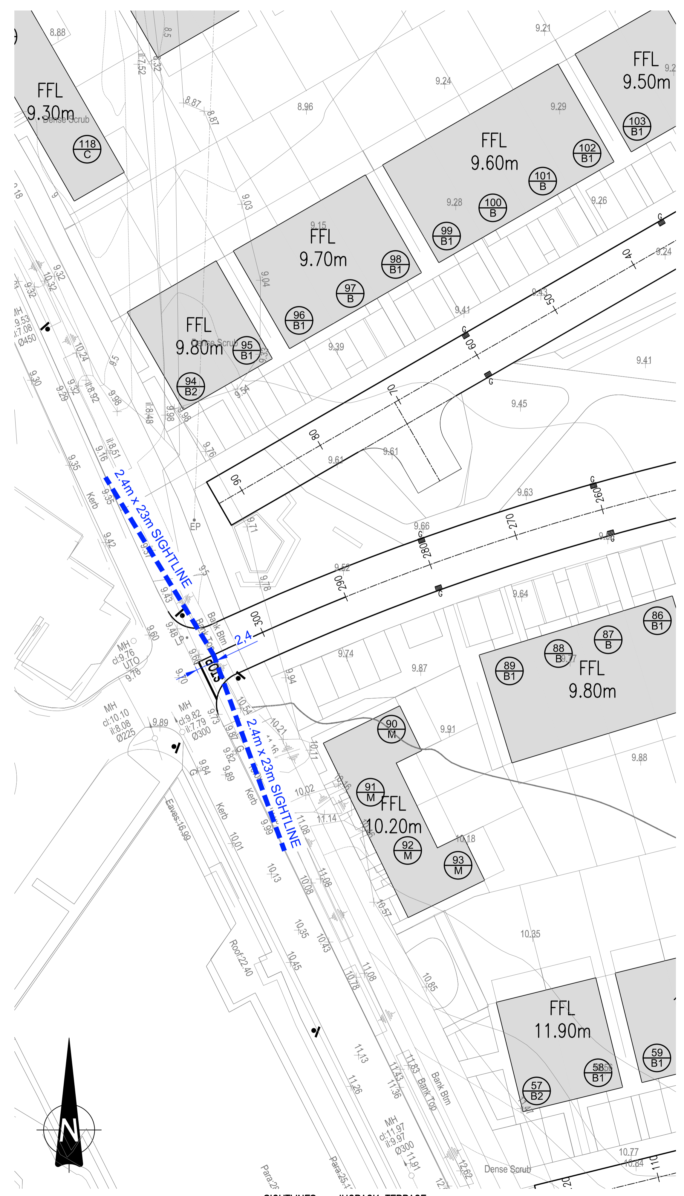
SIGHTLINES – JUGBACK TERRACE SCALE 1:250
